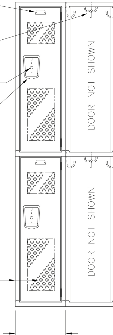
ELEVATION SECTION @ WALL 72" HIGH DOUBLE TIER JORGENSEN VENTILATED LOCKER
