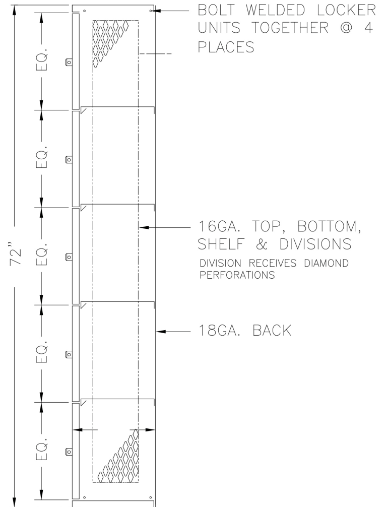
SECTION @ WALL
