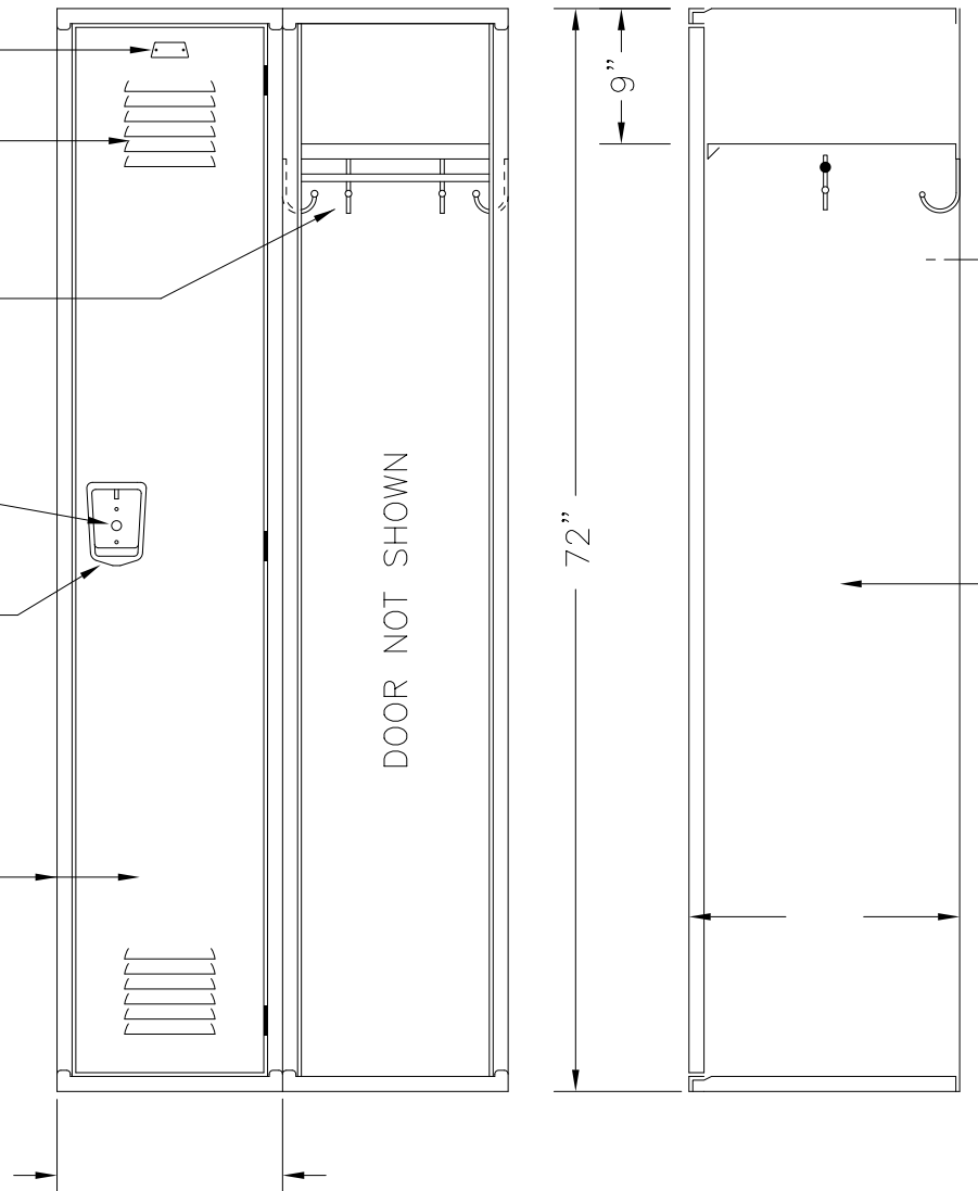
ELEVATION SECTION @ WALL 72" HIGH SINGLE TIER VANGUARD KNOCKDOWN LOCKER W/ RECESSED POCKET
