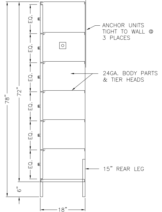
SECTION @ WALL
