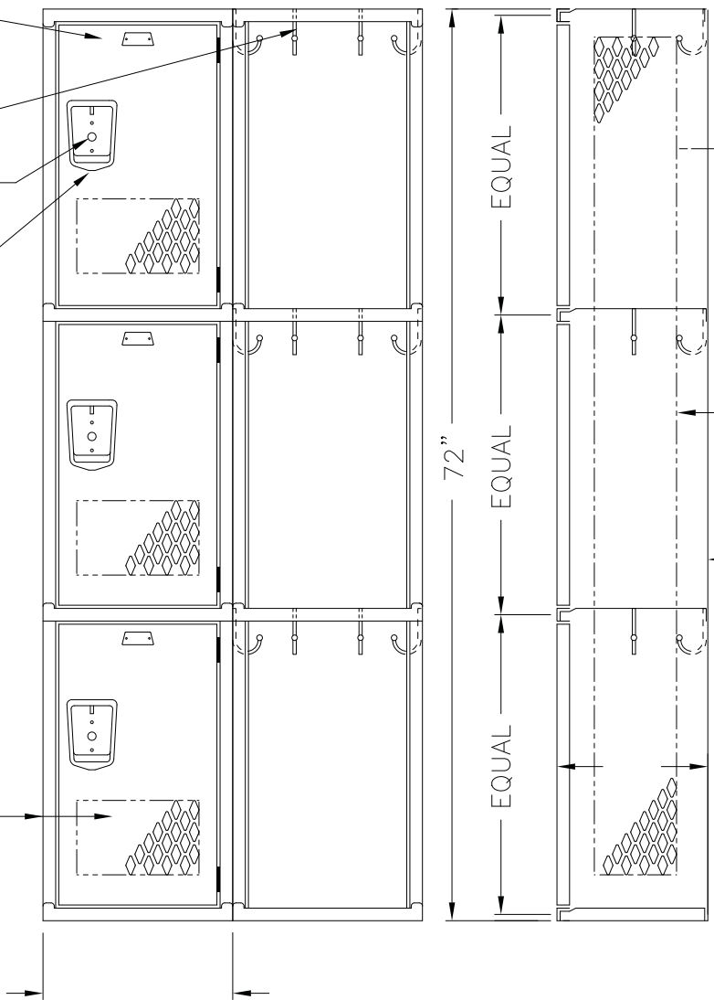
ELEVATION SECTION @ WALL 72" HIGH TRIPLE TIER INVINCIBLE II KNOCKDOWN LOCKER
