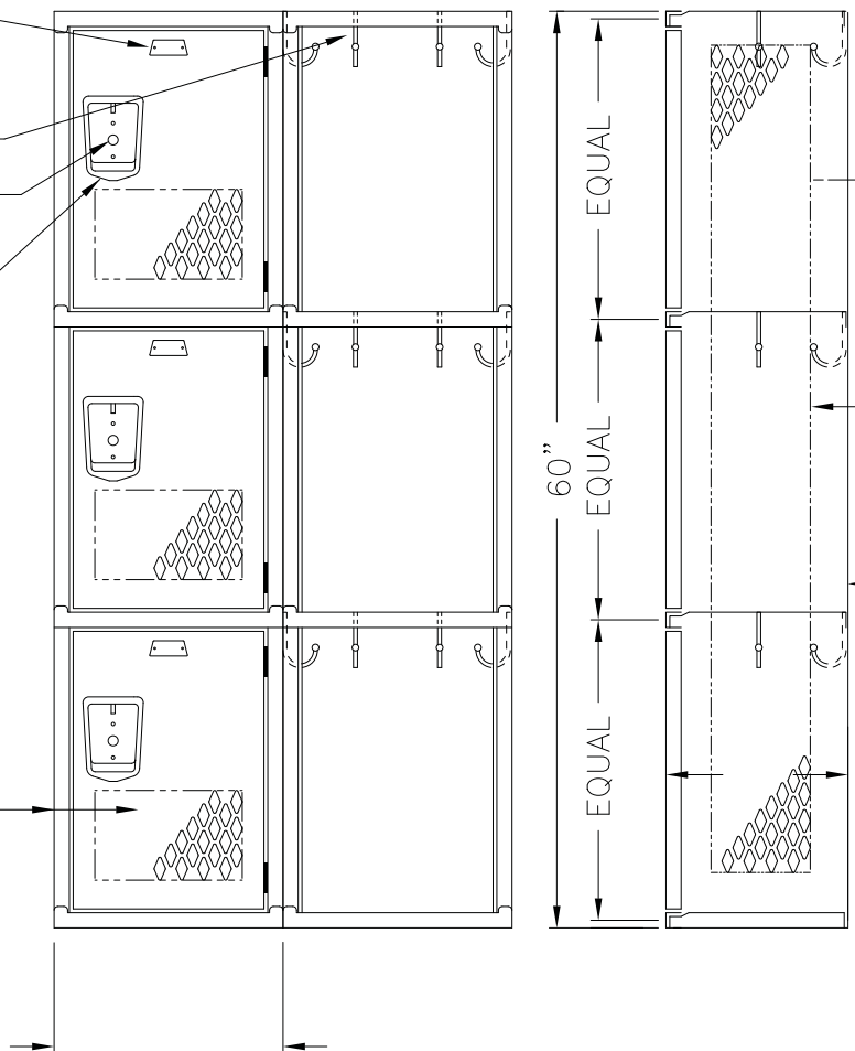
ELEVATION SECTION @ WALL
