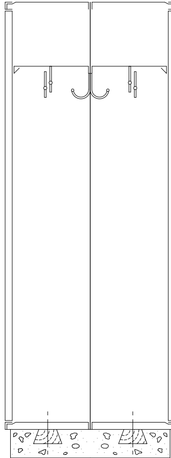
SIDE VIEW @ DBL. ROW
