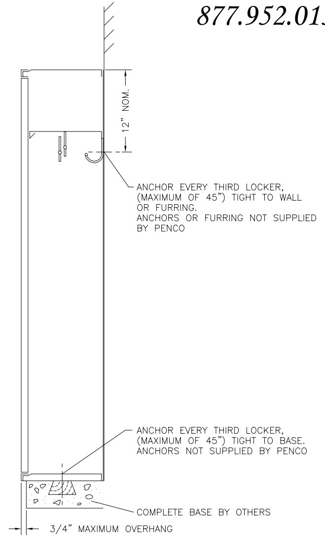
SIDE VIEW @ WALL
