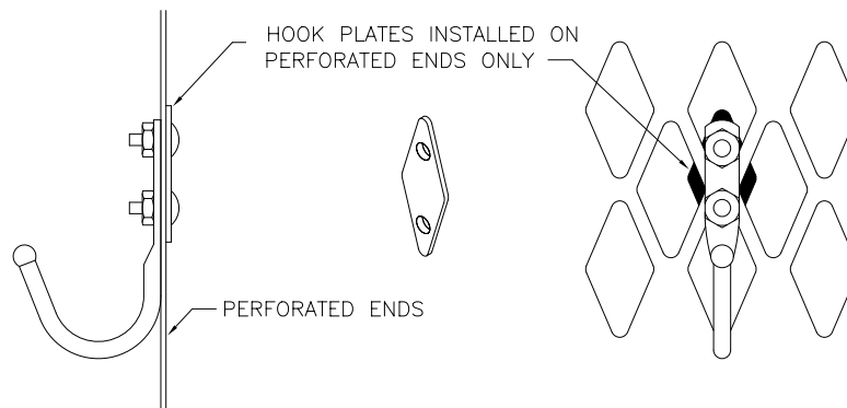
EXPOSED END HOOK ARRANGEMENT
