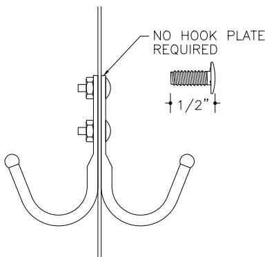
INTERMEDIATE HOOK ARRANGEMENT
