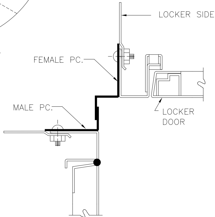
DETAIL © ZEE VERTICAL FILLER
